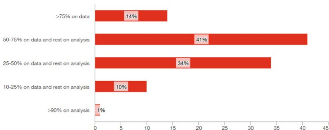
Percentage of time the actuaries spent on data versus analysis and reporting.
